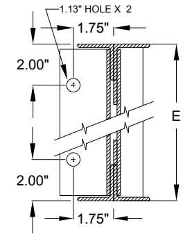
ANCHOR MOUNT DETAIL
