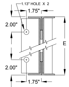
ANCHOR MOUNT DETAIL
