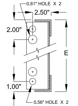
ANCHOR MOUNT DETAIL
